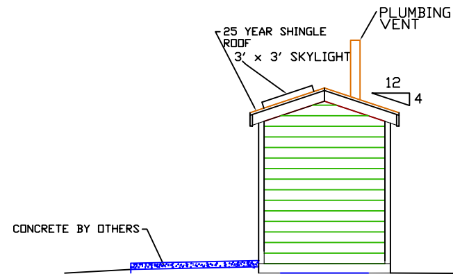
RIGHT ELEV. STANDARD ROOF
