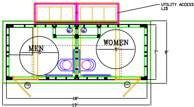
FLOOR PLAN
