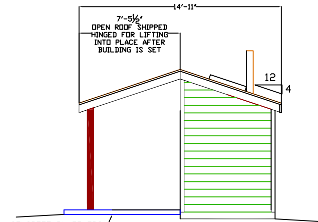
RIGHT ELEV. EXTENDED ROOF KIT
