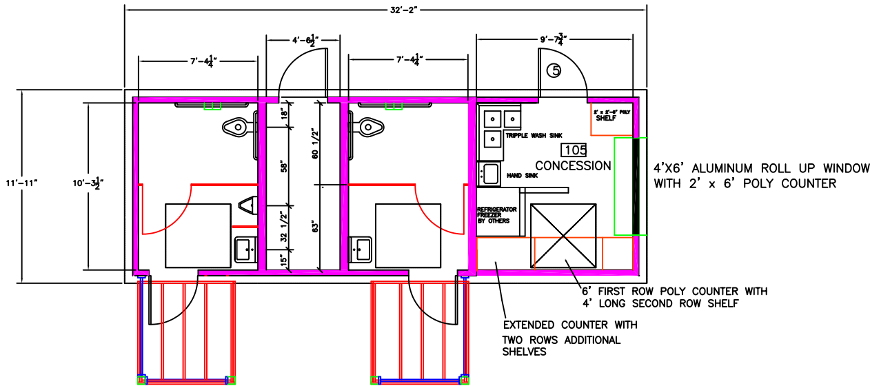
FLOOR PLAN
