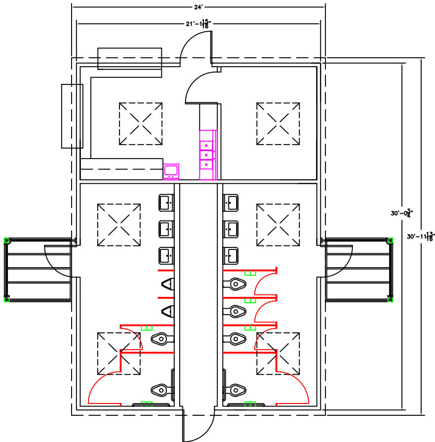
FLOOR PLAN
