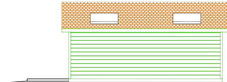
LEFT ELEVATION
