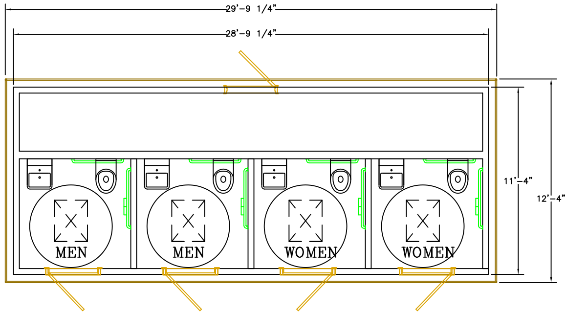
FLOOR PLAN
