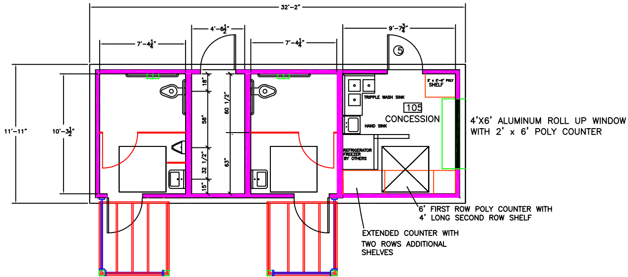
FLOOR PLAN
