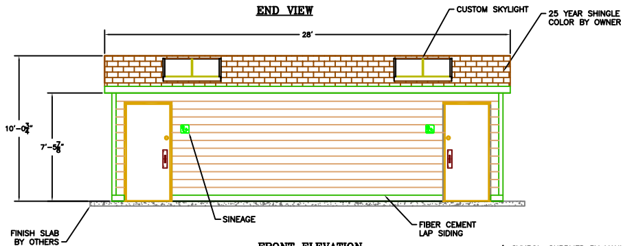
FRONT ELEVATION PRIVACY SCREENS NOT SHOWN
