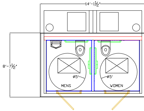
FLOOR PLAN
