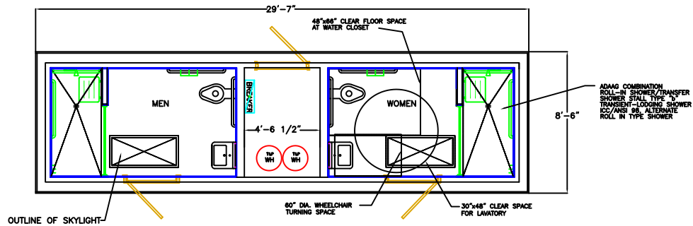
FLOOR PLAN
