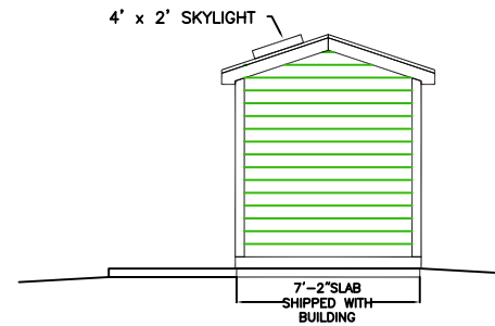
SIDE ELEVATION
