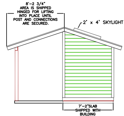
SIDE ELEVATION
