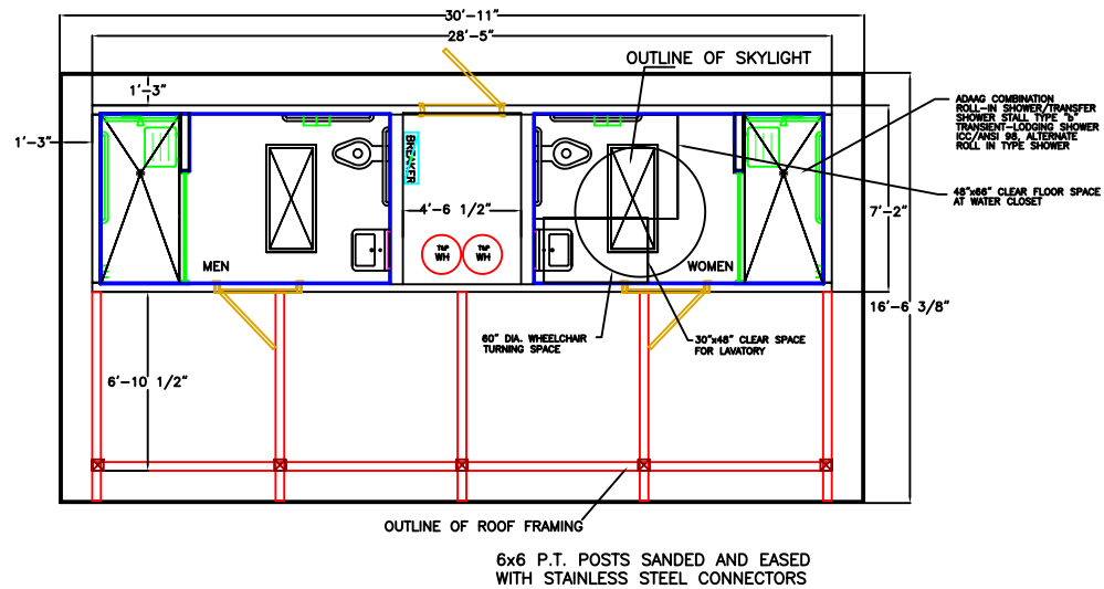
FLOOR PLAN
