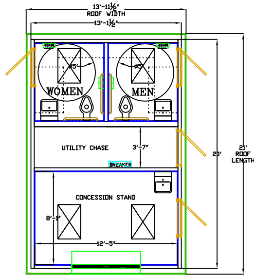
FLOOR PLAN
