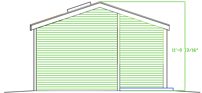
SIDE ELEVATION
