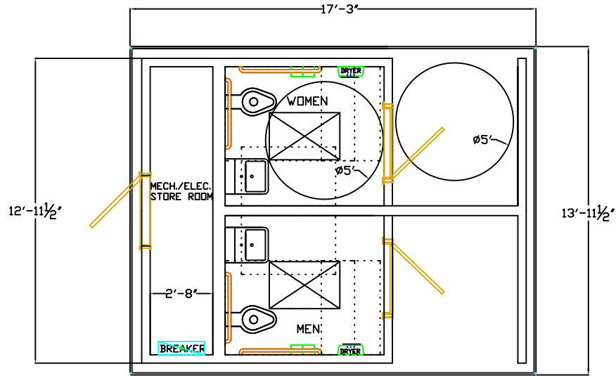
FLOOR PLAN
