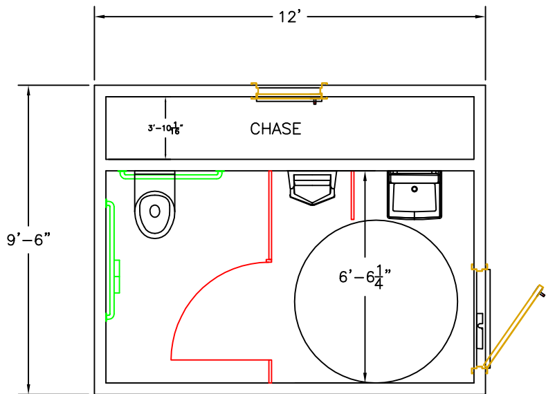
FLOOR PLAN
