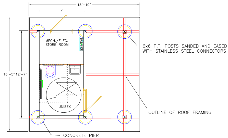
FLOOR PLAN
