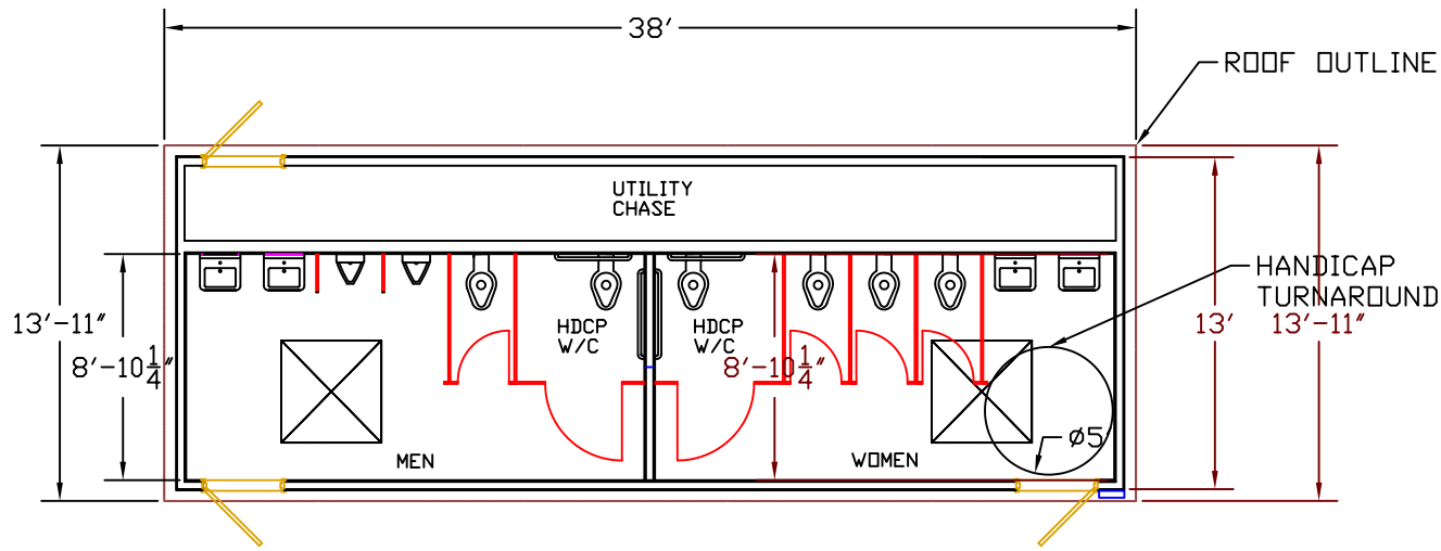
FLOOR PLAN
