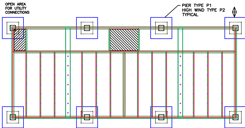
PIER LOCATION PLAN
