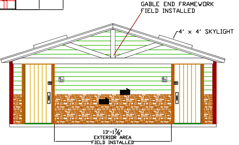
FRONT ELEVATION
