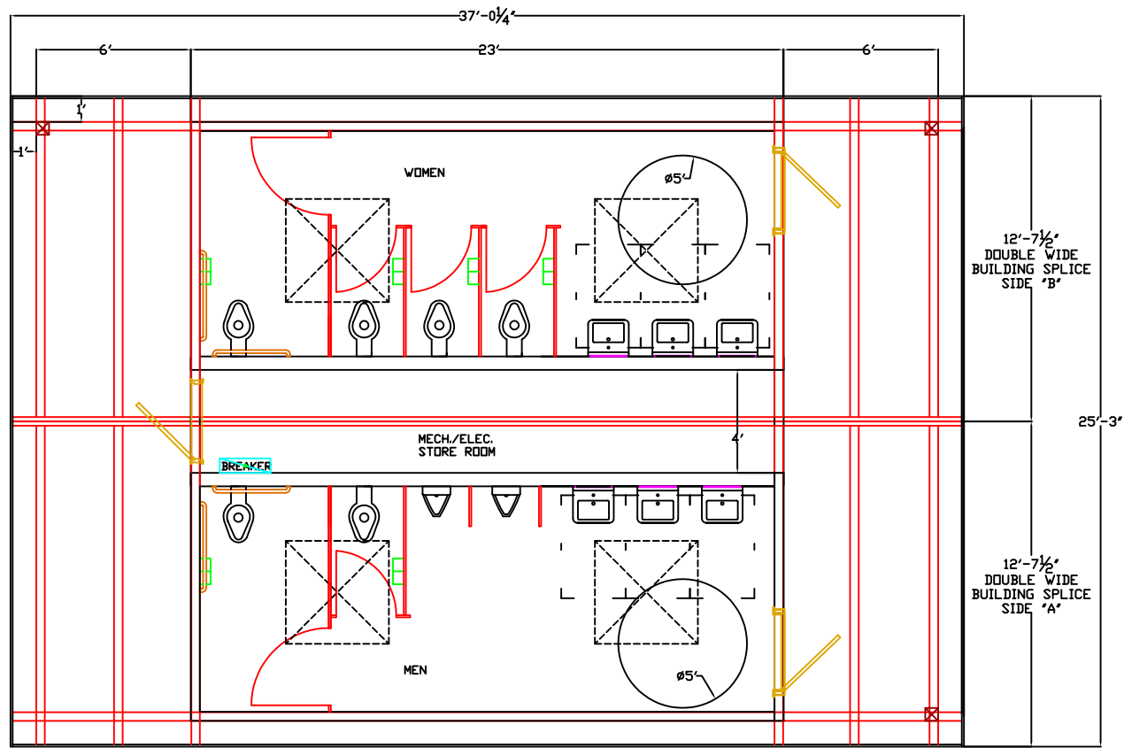
FLOOR PLAN
