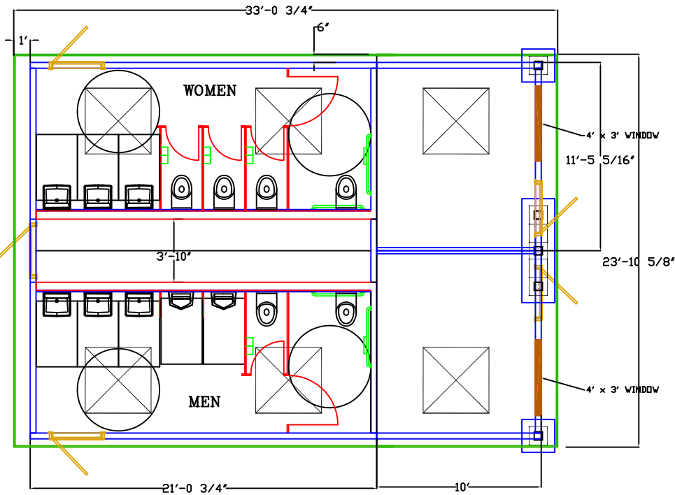
FLOOR PLAN
