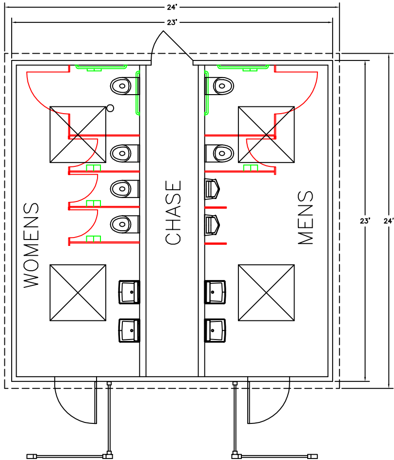
FLOOR PLAN
