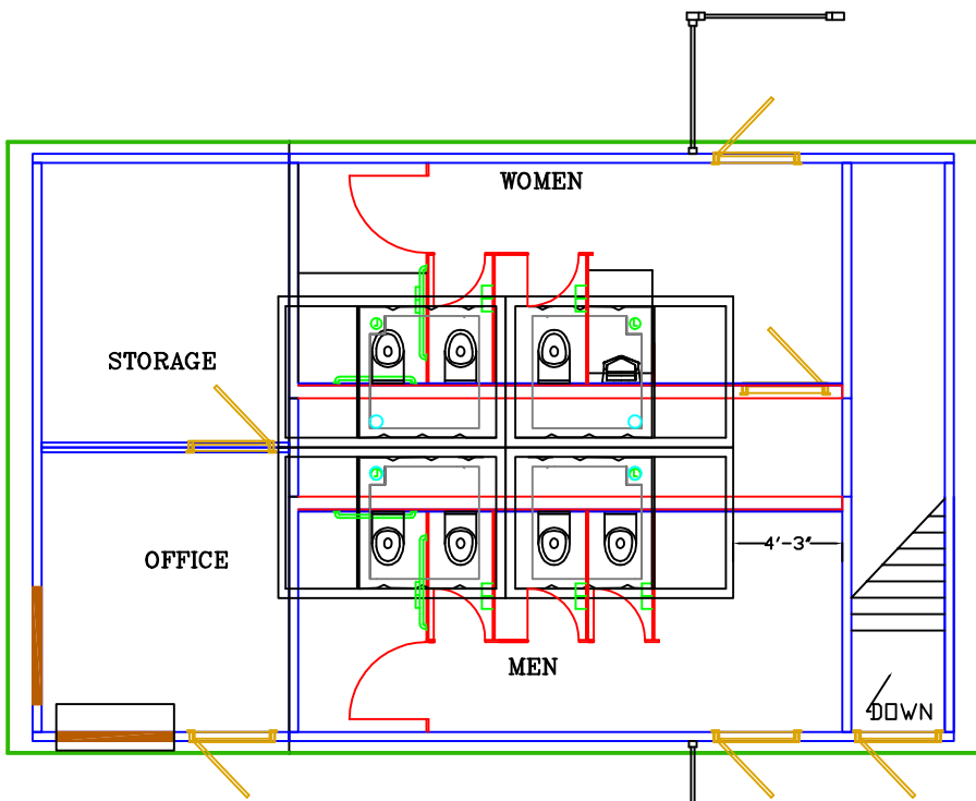
FLOOR PLAN WITH M-32
