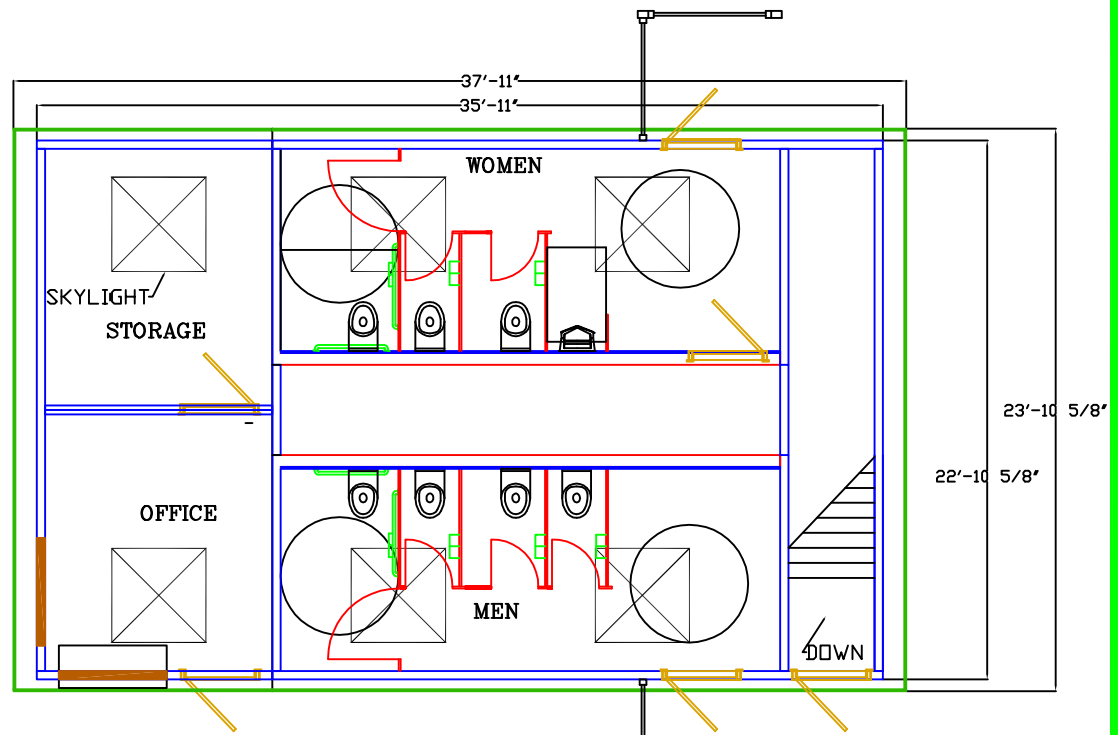
FLOOR PLAN
