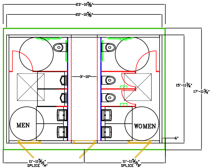
FLOOR PLAN
