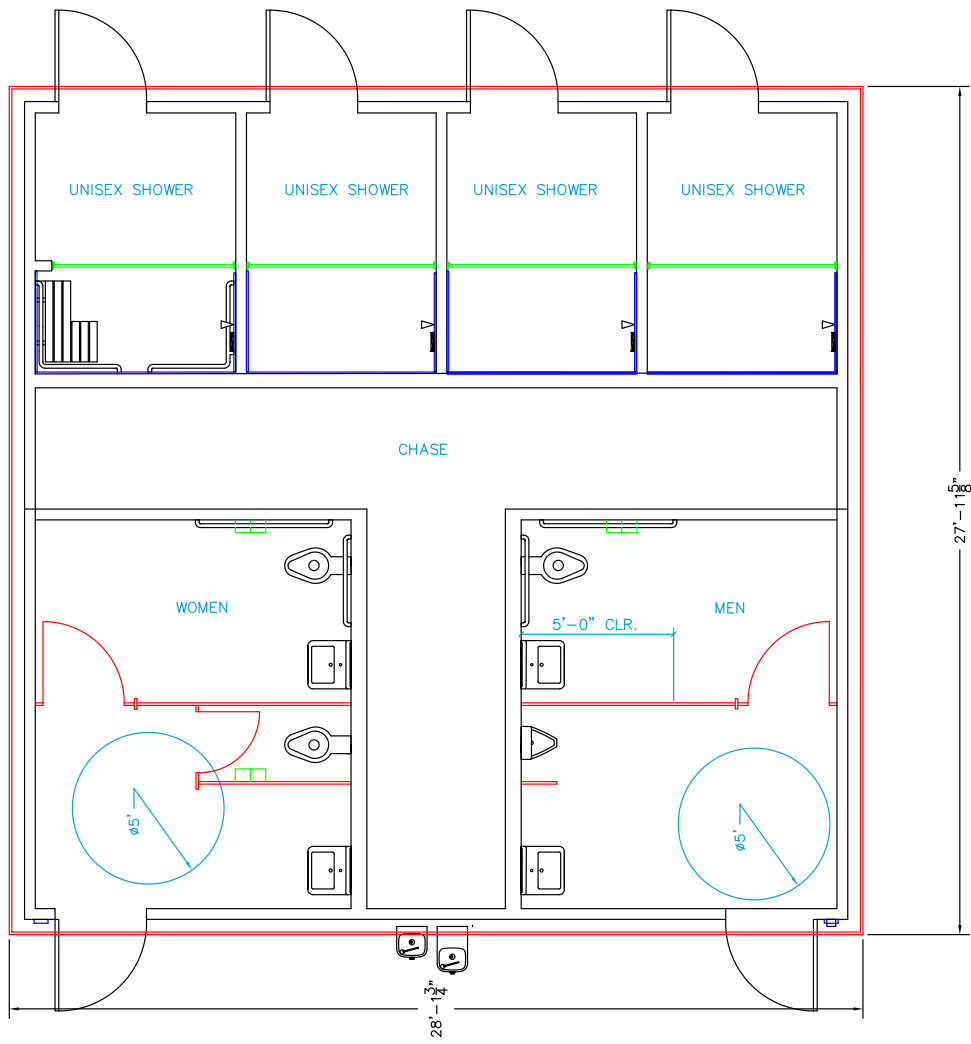
FLOOR PLAN
