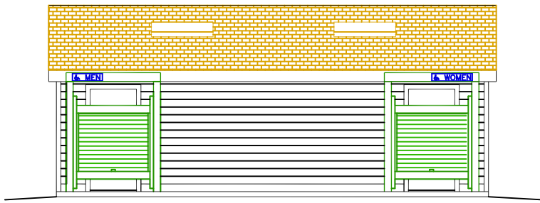
SIDE ELEVATION @ RESTROOM DOOR
