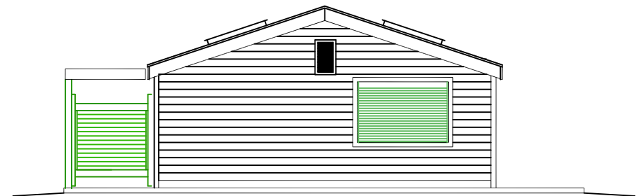
END ELEVATION @ CONCESSION WINDOW
