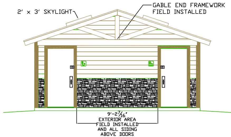
FRONT ELEVATION
