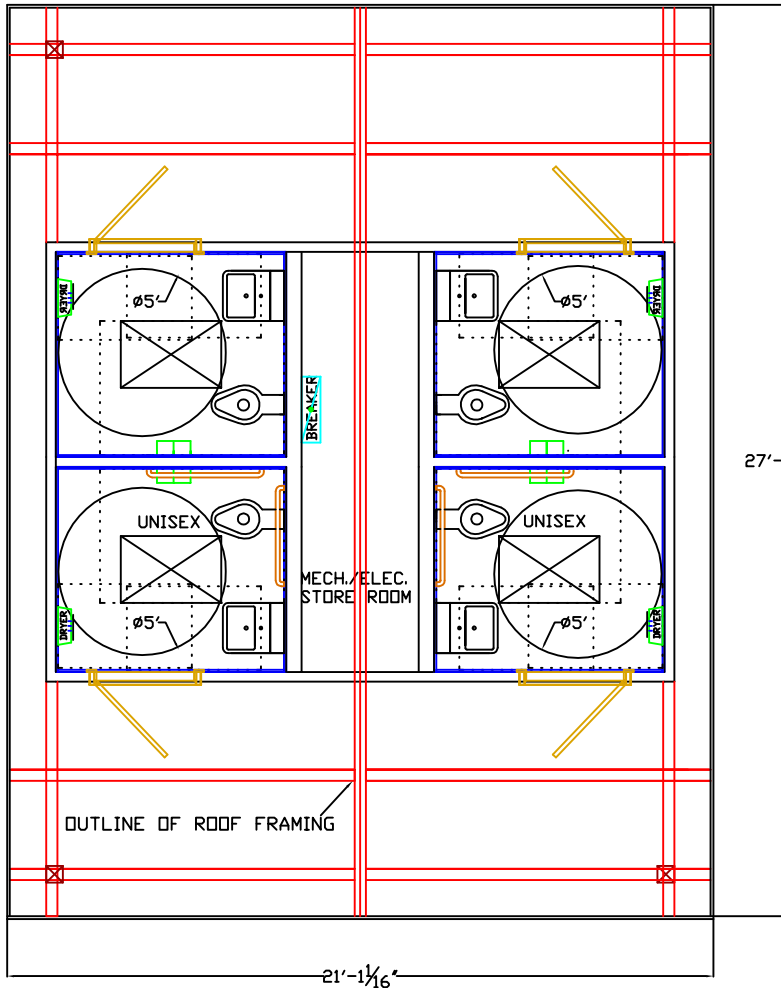
FLOOR PLAN
