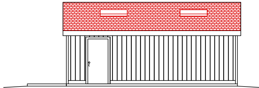
SIDE ELEVATION @ CONCESSION DOOR
