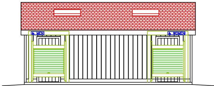
SIDE ELEVATION @ RESTROOM DOOR
