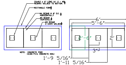
P4 PLAN VIEW @ PIER
