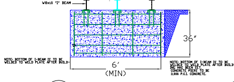
P4 SECTION DETAIL @ PIER
