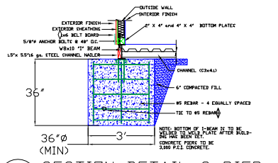
P2 SECTION DETAIL @ PIER
