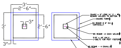
P2 PLAN VIEW @ PIER
