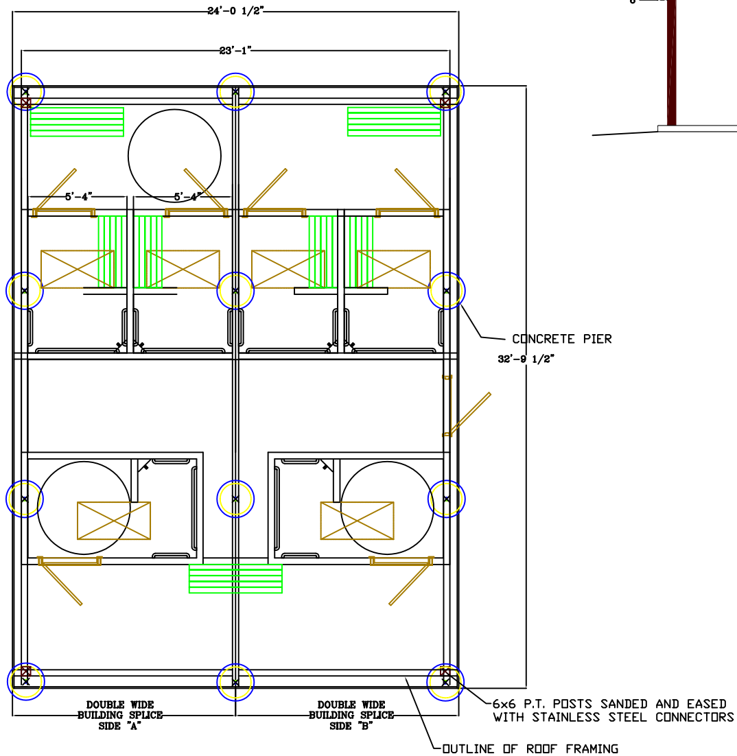
FLOOR PLAN
