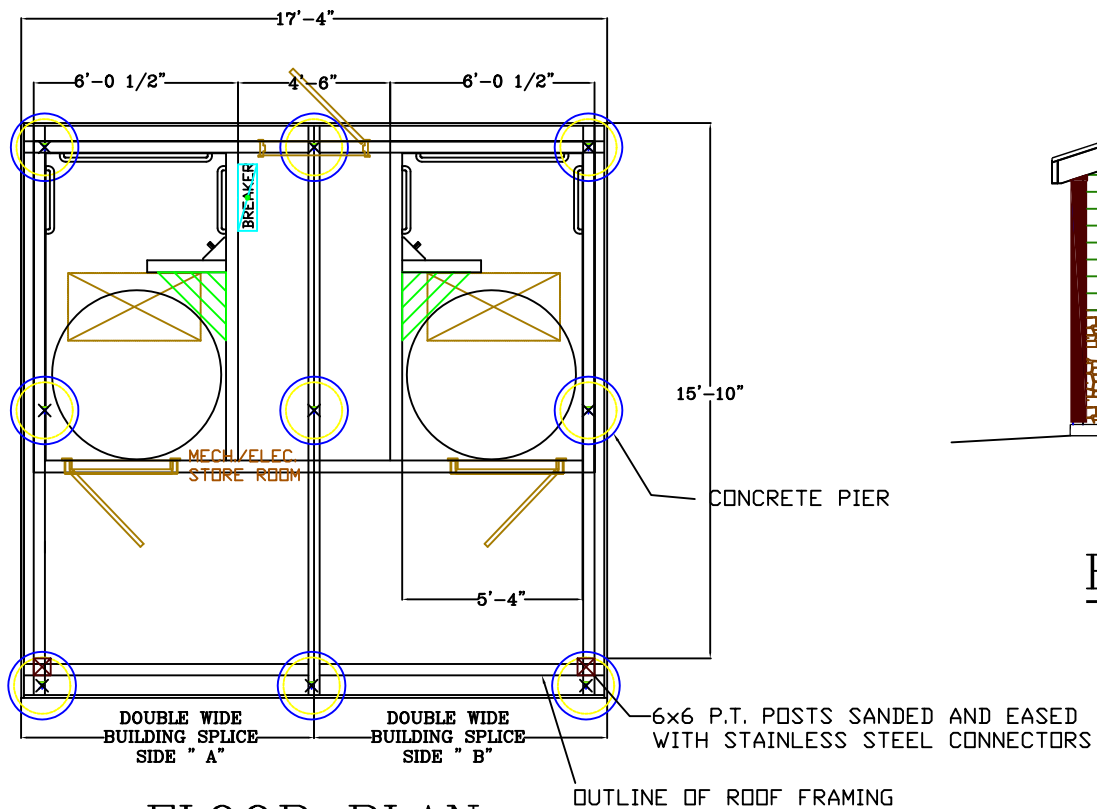
FLOOR PLAN
