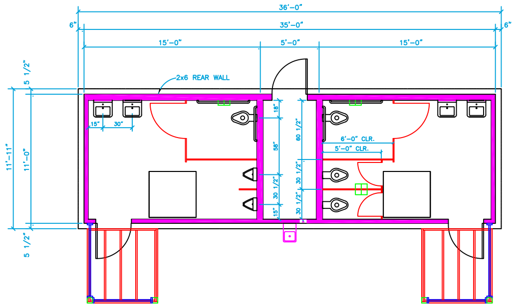
FLOOR PLAN
