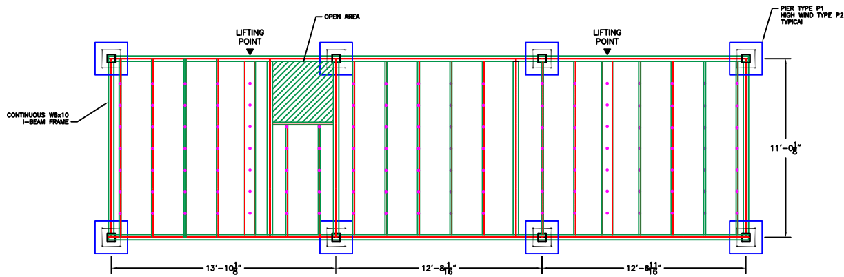
PIER LOCATION PLAN
