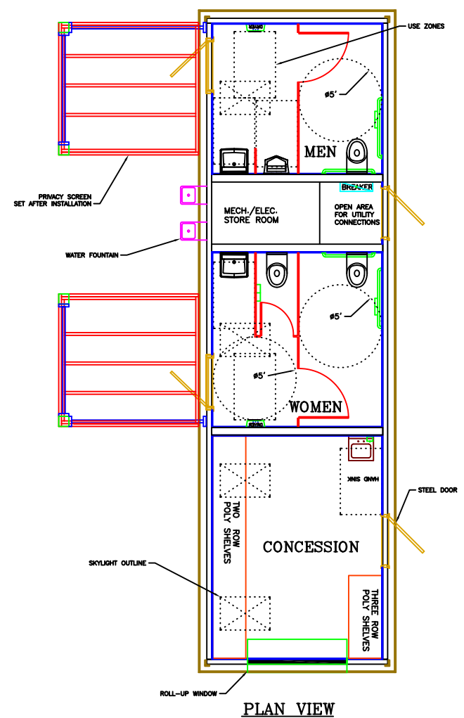
PLAN VIEW
