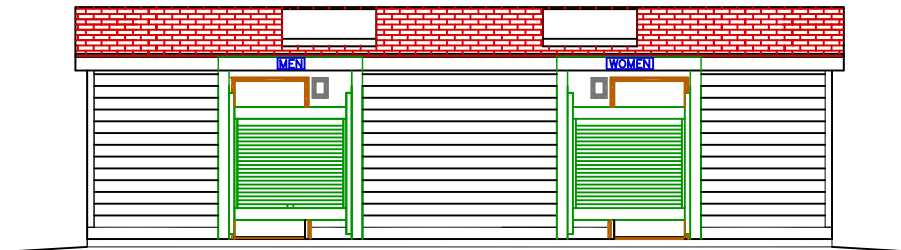
FRONT ELEVATION
