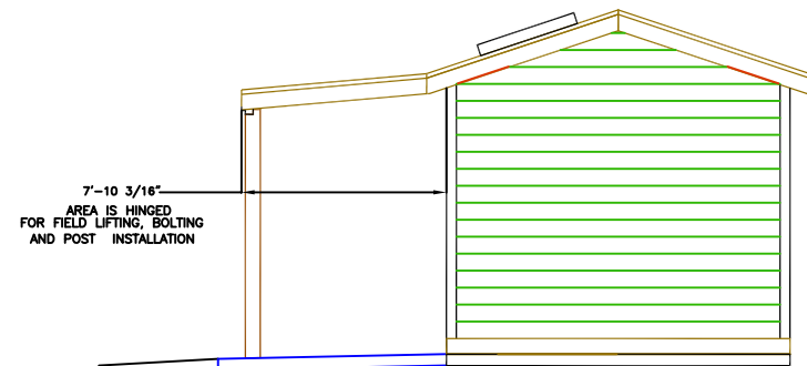
SIDE ELEVATION
