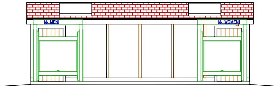
FRONT ELEVATION
