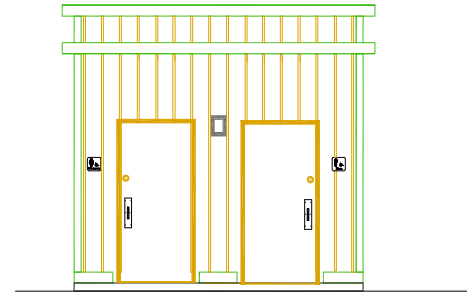
FRONT ELEVATION
