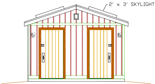
FRONT ELEVATION OPTIONAL ROOF PACKAGE (REV)
