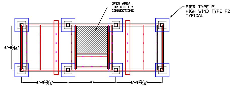
PIER LOCATION PLAN
