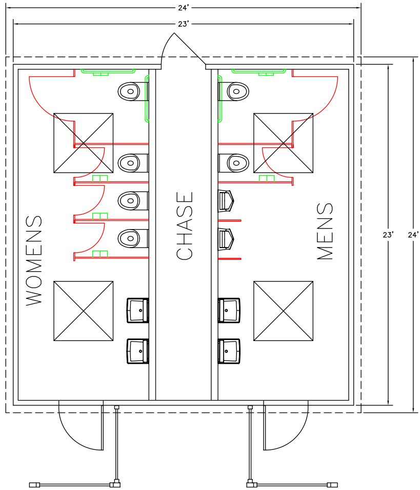
FLOOR PLAN
