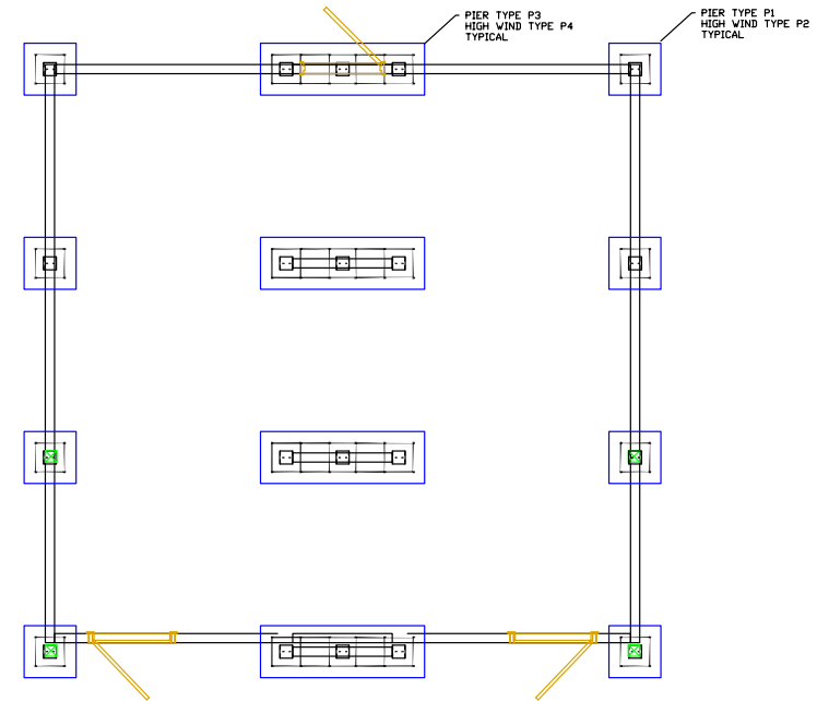
PIER LOCATION PLAN \diamond
